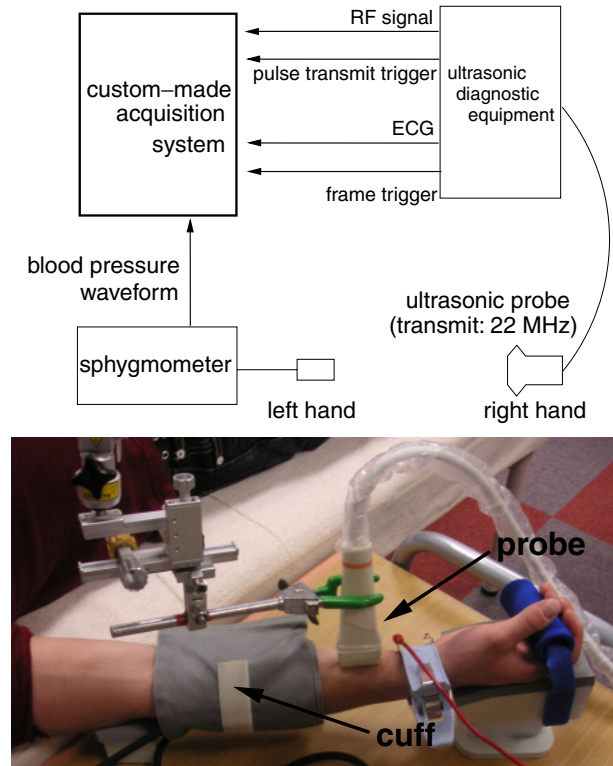
Fig. 1. (Color online) Ultrasonic measurement of radial artery.
