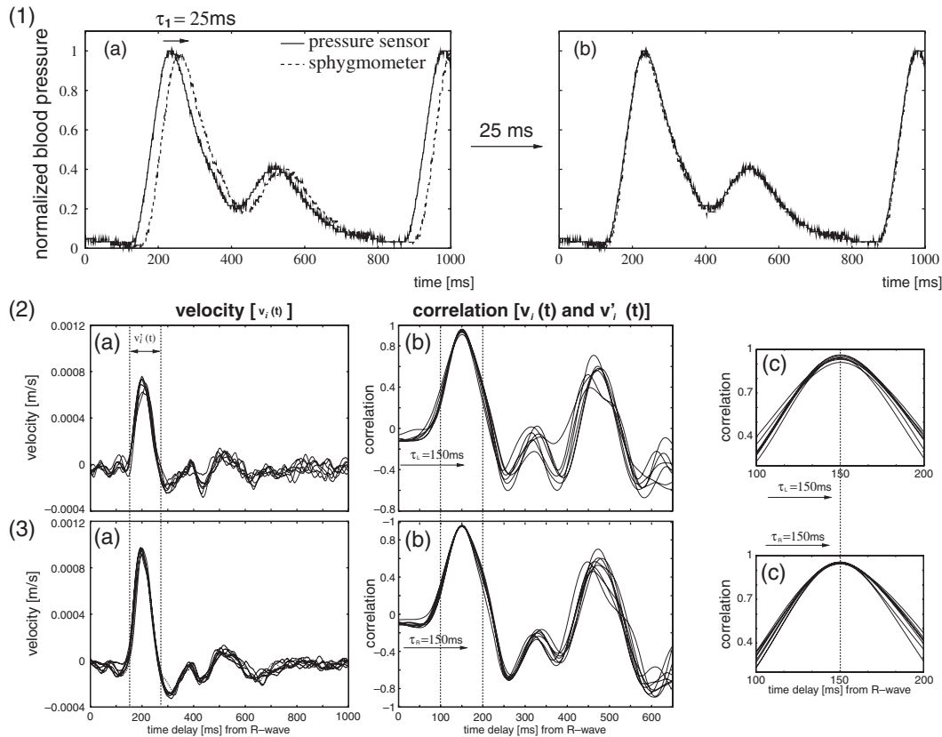
Fig. 2. (1) Correction of delay caused by experimental system. For (2) left and (3) right radial arteries, (a) velocities of arterial walls, (b) correlation functions, and (c) enlarged views of (b).
